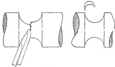
FIG. 125. SMALL GOUGE IN ACTION.
